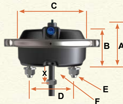
C30L3 (shown)
